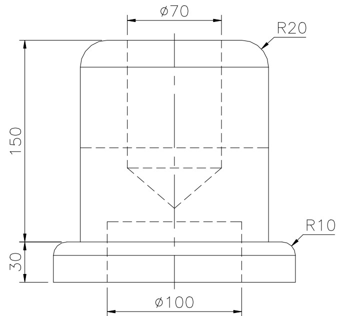
RIGHT SCALE 1/3
