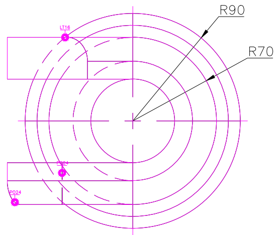
TOP SCALE 1/3
