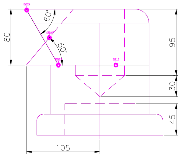
FRONT SCALE 1/3
