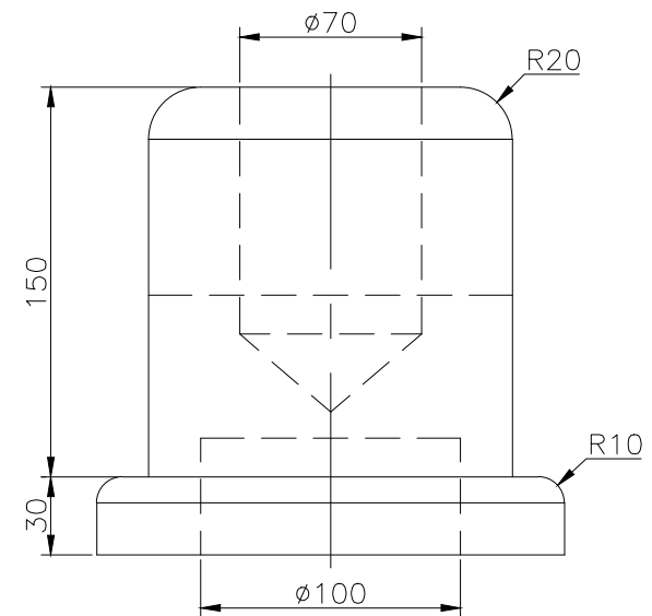
RIGHT SCALE 1/3
