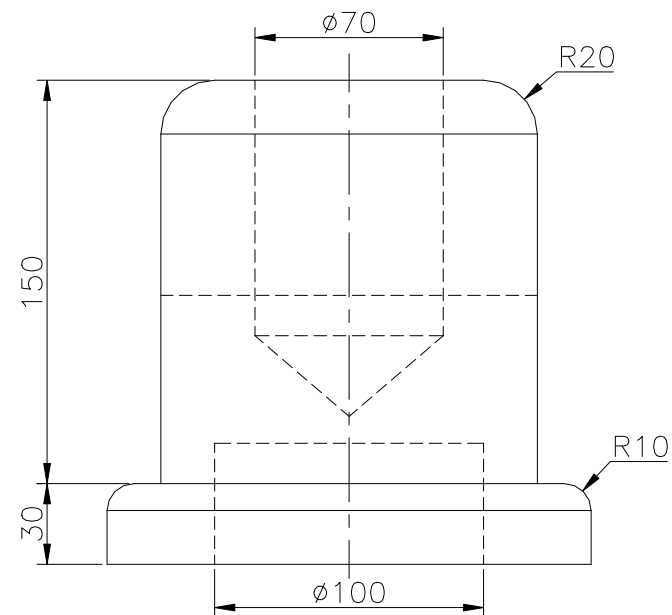
RIGHT SCALE 1/3
