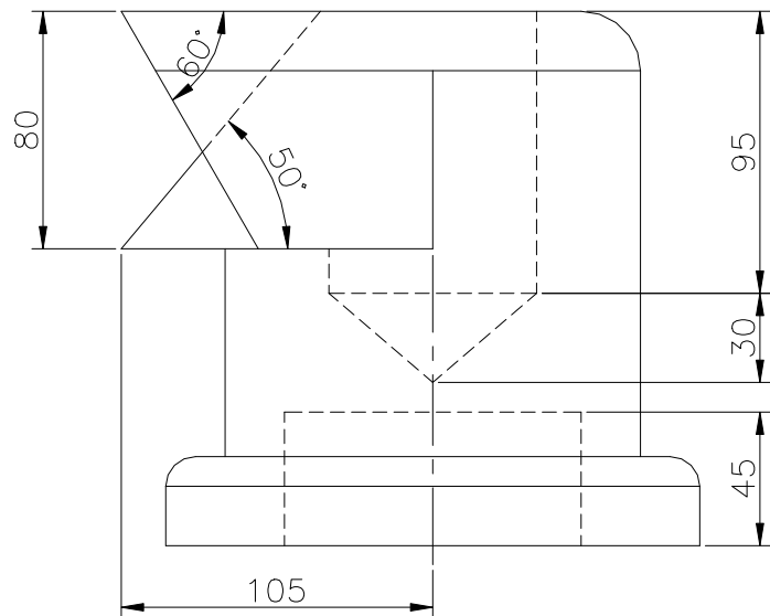
FRONT SCALE 1/3
