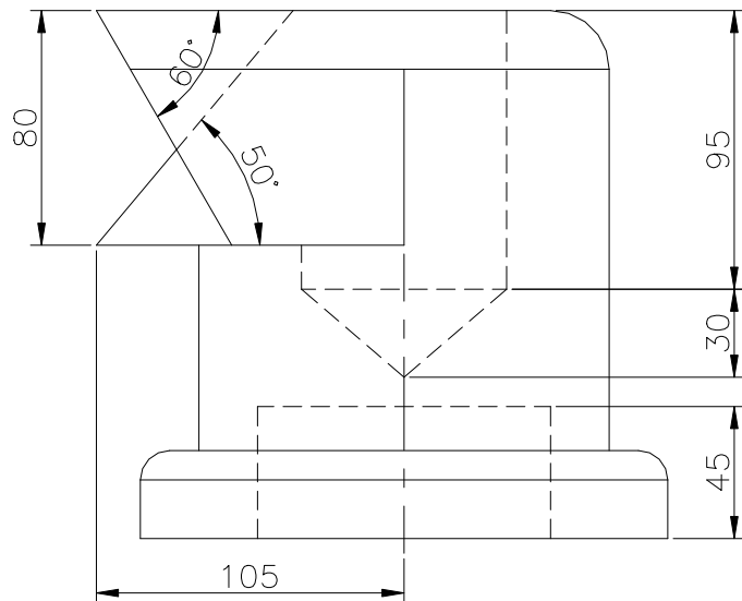
FRONT SCALE 1/3
