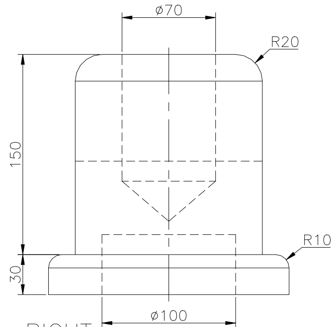
RIGHT SCALE 1/3
