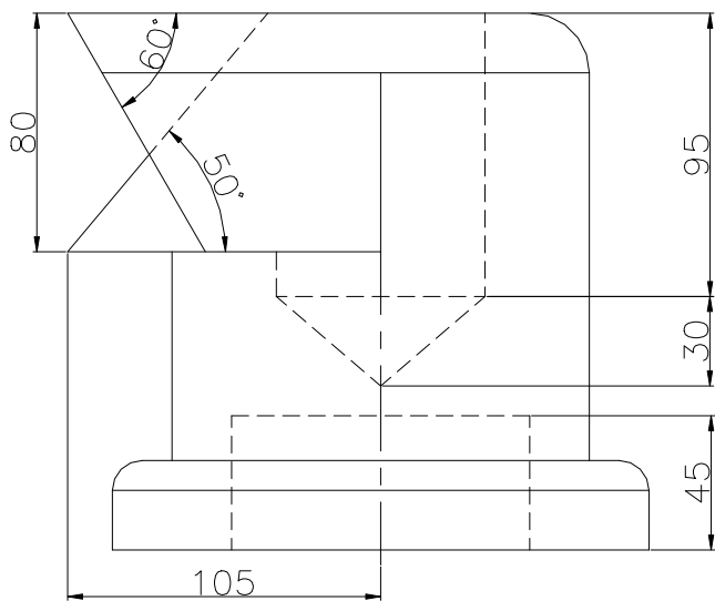
FRONT SCALE 1/3
