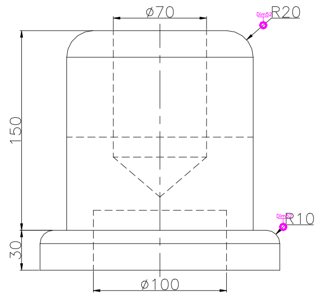
RIGHT SCALE 1/3
