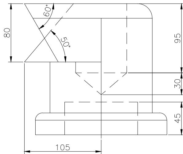
FRONT SCALE 1/3
