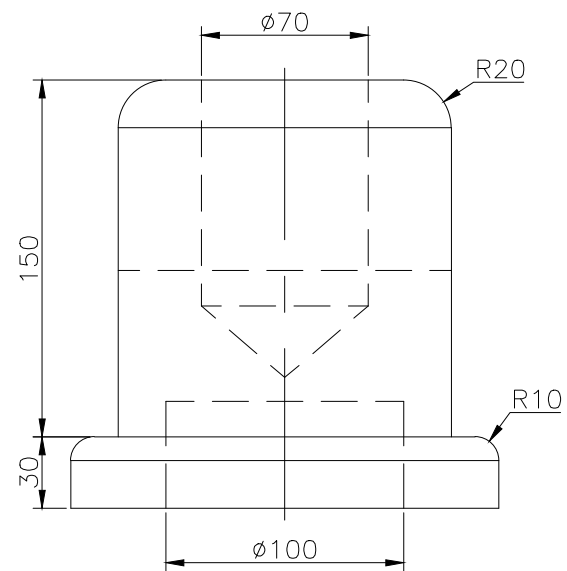
RIGHT SCALE 1/3
