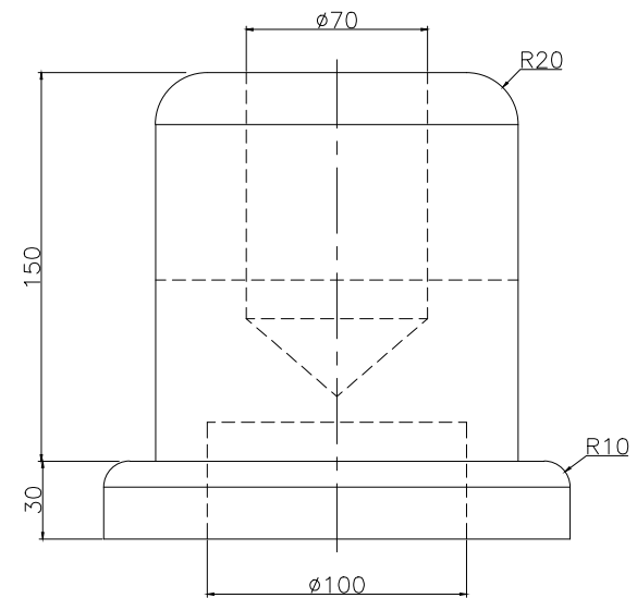
RIGHT SCALE 1/3
