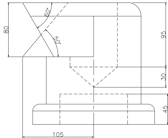
FRONT SCALE 1/3
