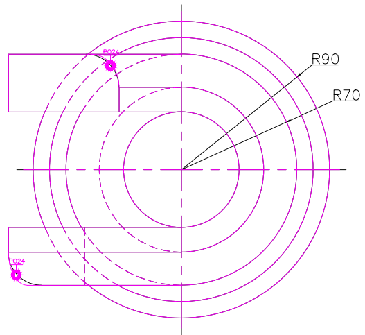
TOP SCALE 1/3
