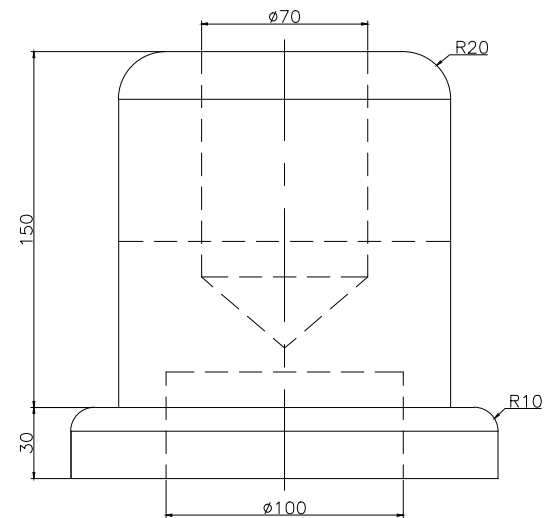
RIGHT SCALE 1/3
