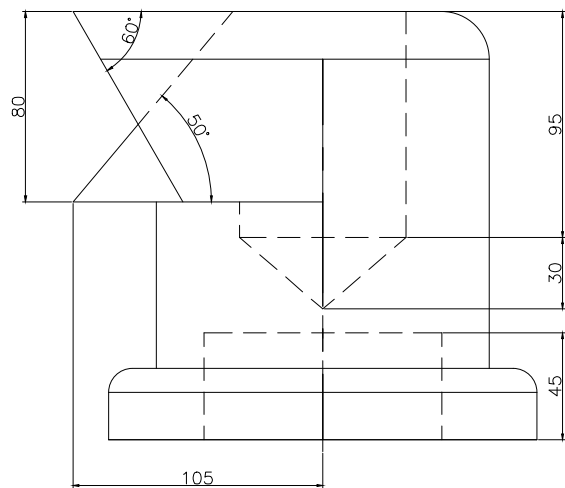
FRONT SCALE 1/3
