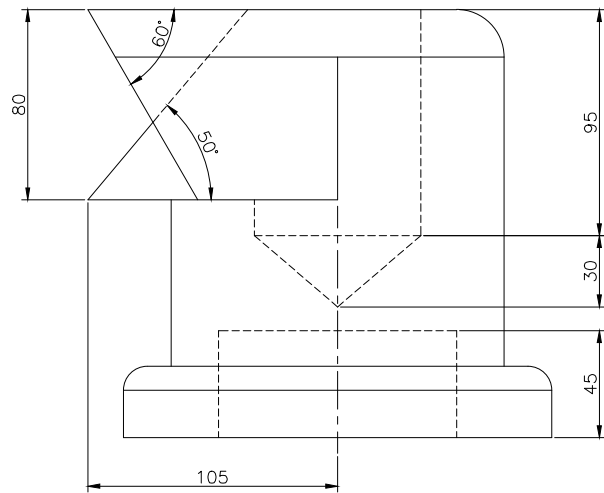
FRONT SCALE 1/3
