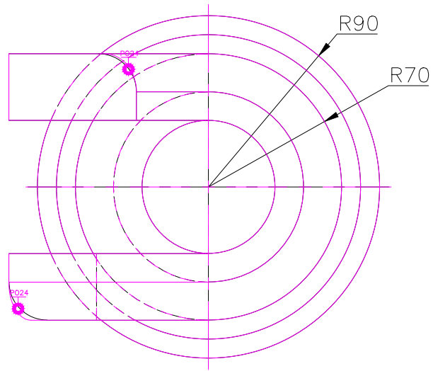
TOP SCALE 1/3
