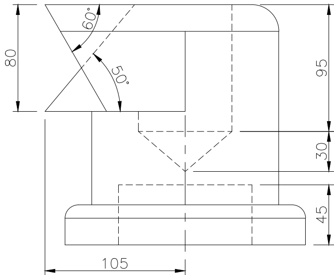
FRONT SCALE 1/3
