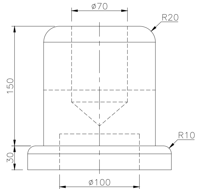
RIGHT SCALE 1/3
