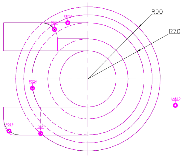
TOP SCALE 1/3
