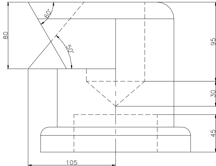
FRONT SCALE 1/3
