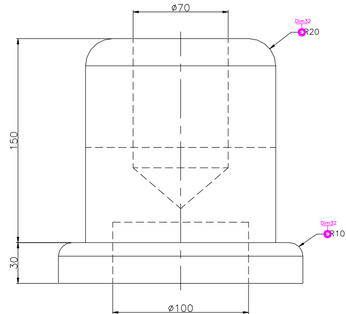
RIGHT SCALE 1/3
