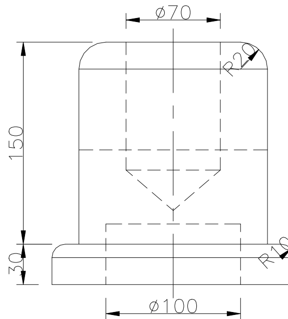
RIGHT SCALE 1/3
