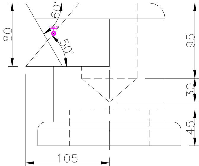
FRONT SCALE 1/3
