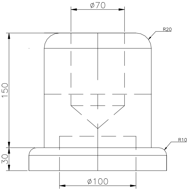
RIGHT SCALE 1/3
