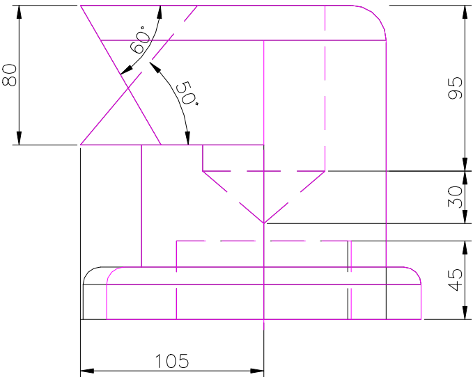
FRONT SCALE 1/3
