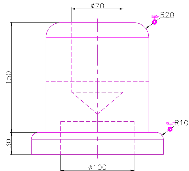
RIGHT SCALE 1/3
