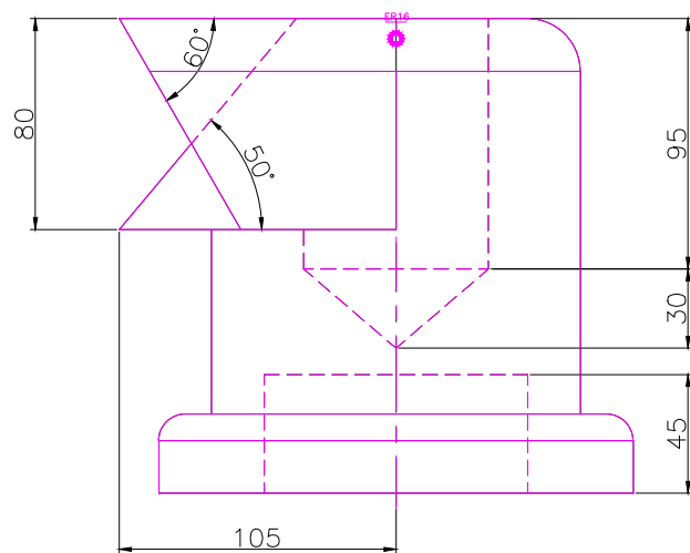
FRONT SCALE 1/3
