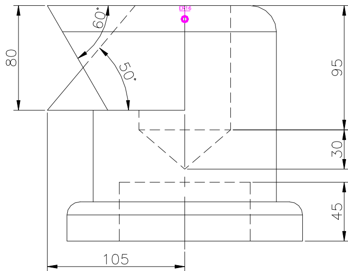
FRONT SCALE 1/3
