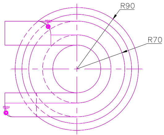
TOP SCALE 1/3
