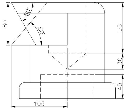
FRONT SCALE 1/3
