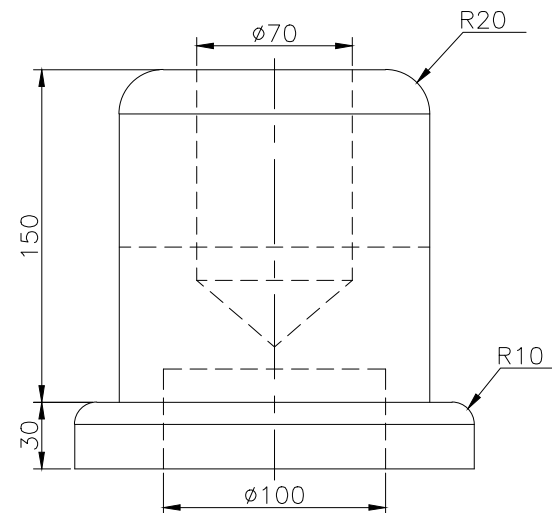
RIGHT SCALE 1/3
