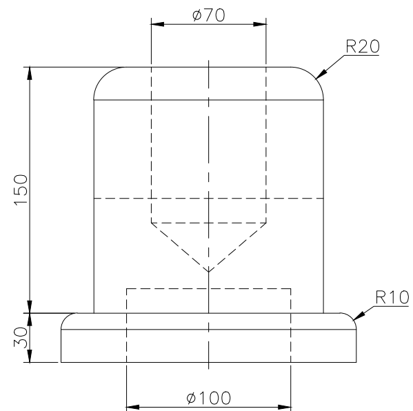
RIGHT SCALE 1/3
