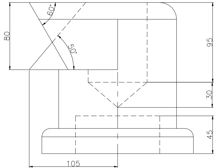
FRONT SCALE 1/3
