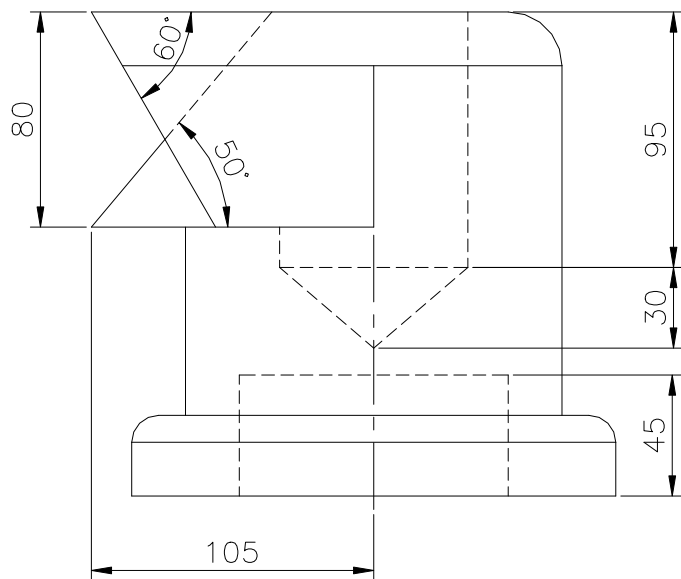
FRONT SCALE 1/3
