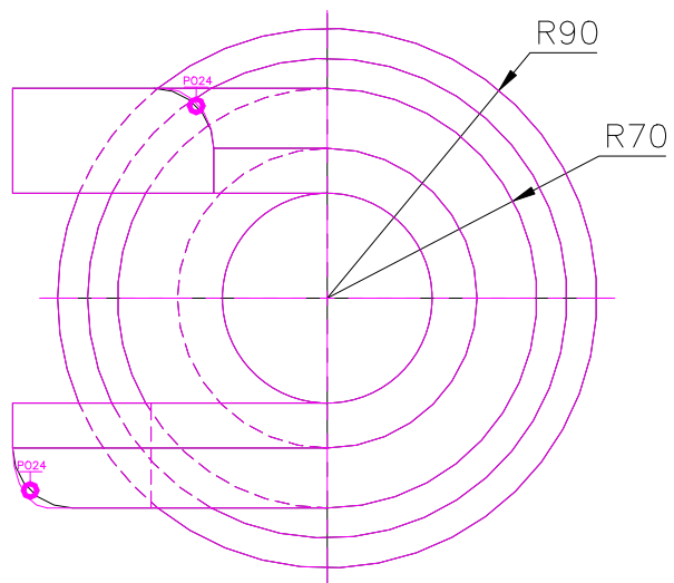
TOP SCALE 1/3
