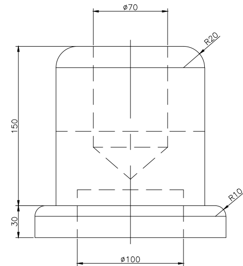
RIGHT SCALE 1/3
