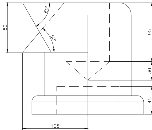
FRONT SCALE 1/3
