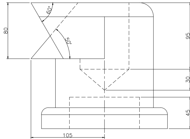
FRONT SCALE 1/3
