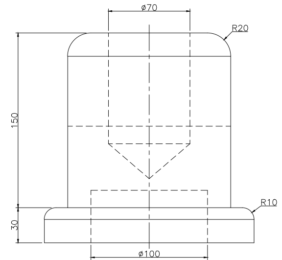
RIGHT SCALE 1/3
