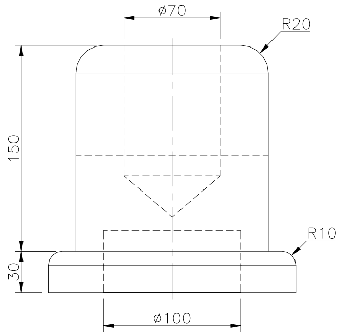
RIGHT SCALE 1/3
