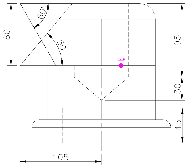
FRONT SCALE 1/3
