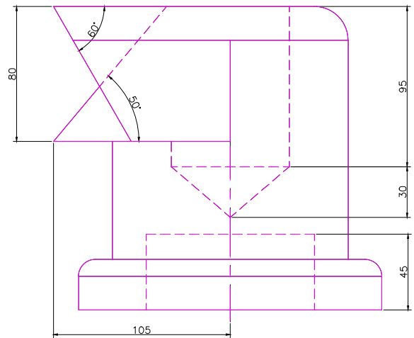
FRONT SCALE 1/3
