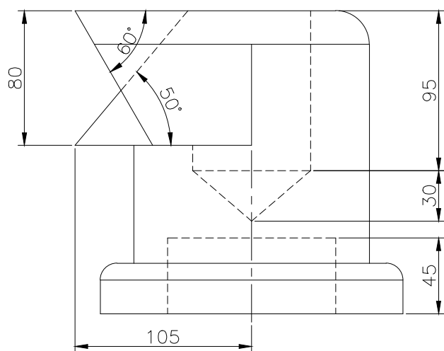
FRONT SCALE 1/3
