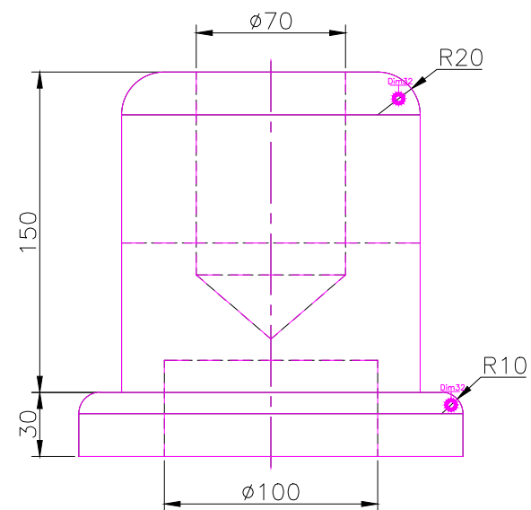
RIGHT SCALE 1/3
