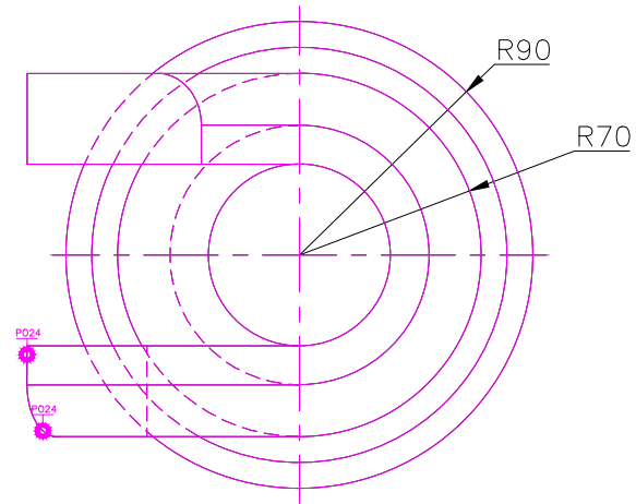
TOP SCALE 1/3
