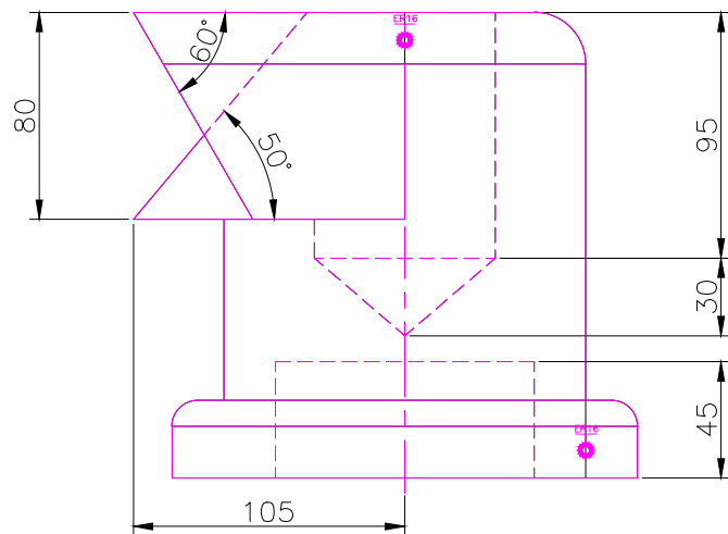
FRONT SCALE 1/3
