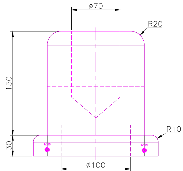
RIGHT SCALE 1/3
