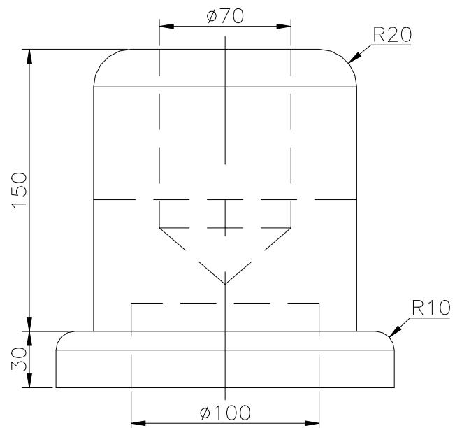
RIGHT SCALE 1/3
