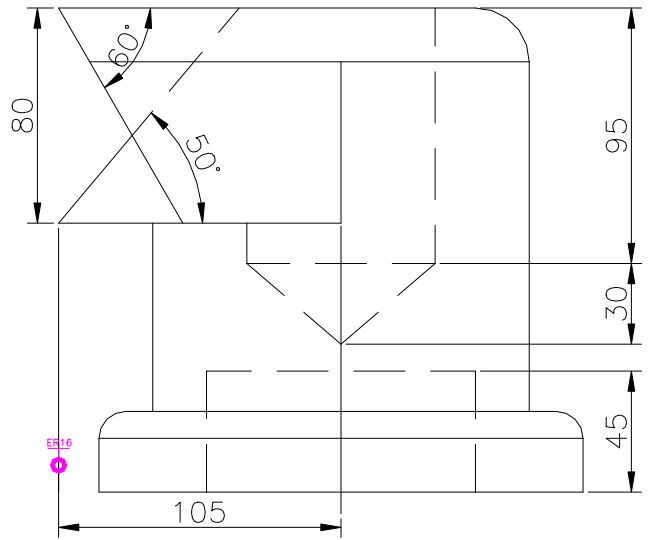
FRONT SCALE 1/3
