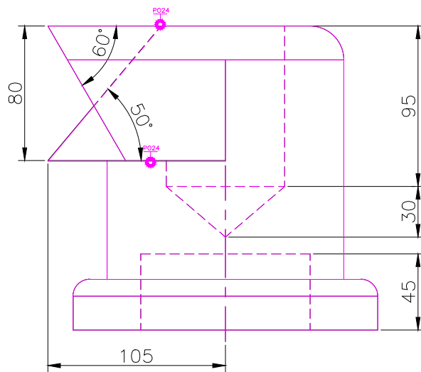
FRONT SCALE 1/3
