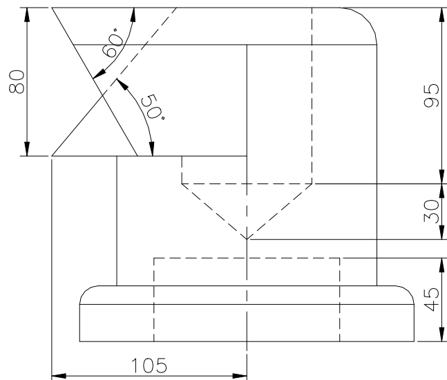
FRONT SCALE 1/3
