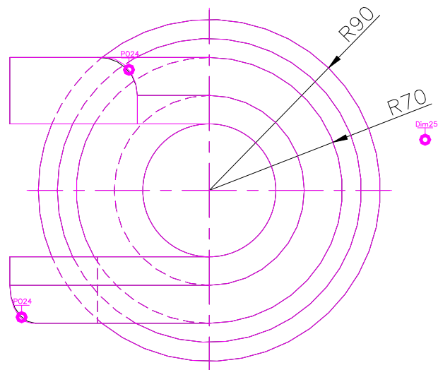
TOP SCALE 1/3
