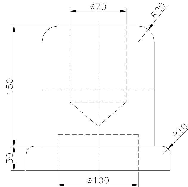
RIGHT SCALE 1/3
