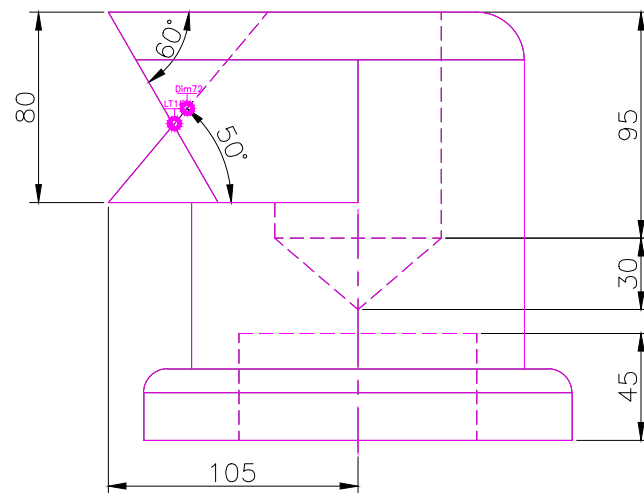
FRONT SCALE 1/3
