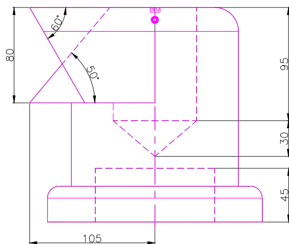
FRONT SCALE 1/3
