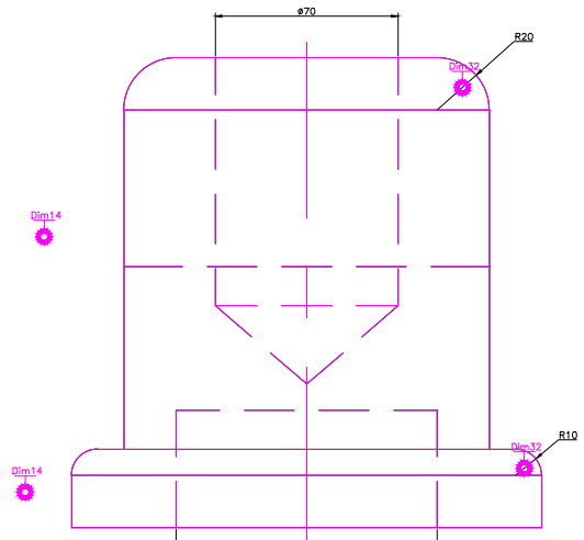
RIGHT SCALE 1/3
