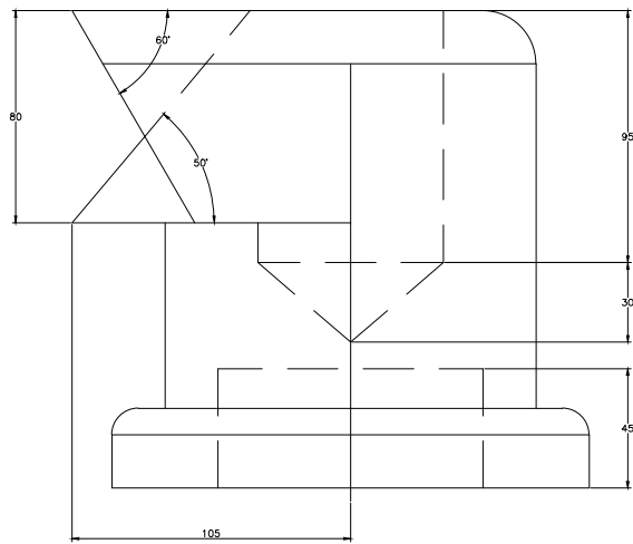
FRONT SCALE 1/3
