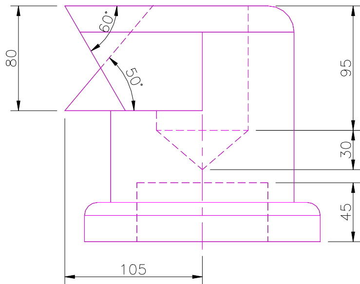
FRONT SCALE 1/3
