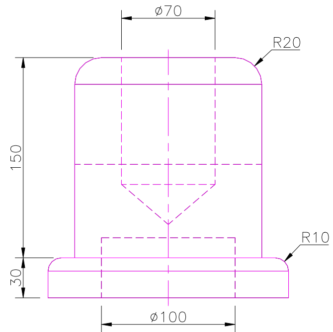
RIGHT SCALE 1/3
