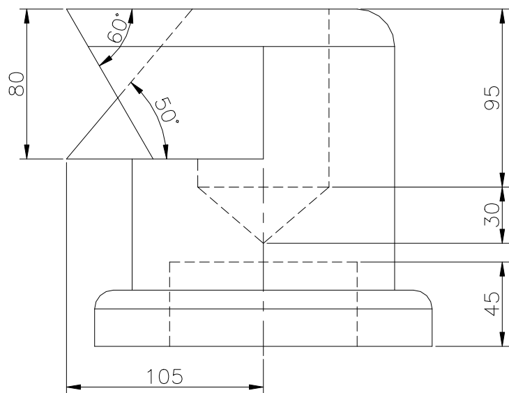
FRONT SCALE 1/3
