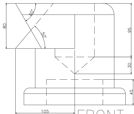
FRONT SCALE 1/3
