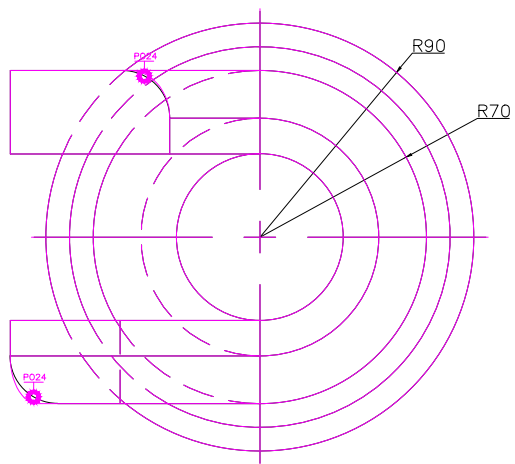
TOP SCALE 1/3
