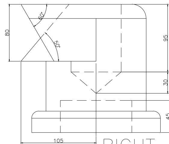
RIGHT SCALE 1/3
