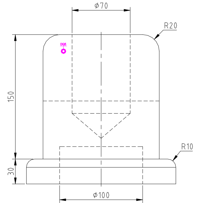
RIGHT SCALE 1/3
