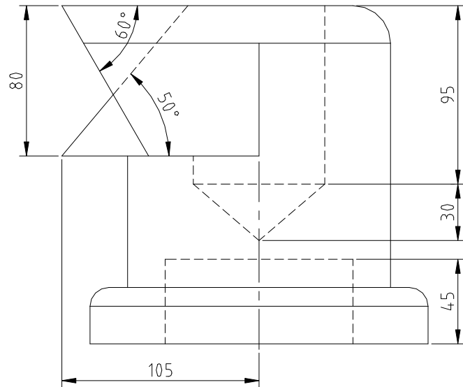
FRONT SCALE 1/3
