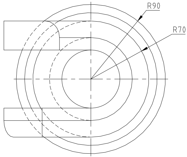
TOP SCALE 1/3
