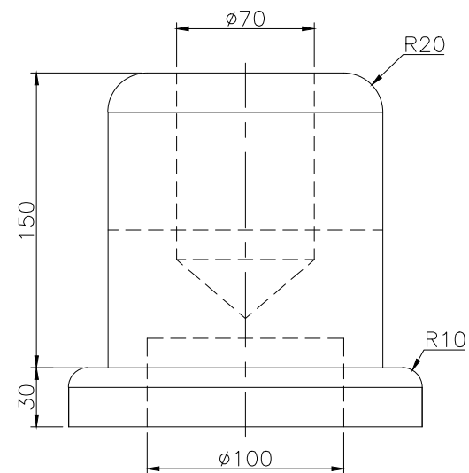
RIGHT SCALE 1/3
