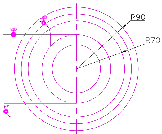
TOP SCALE 1/3
