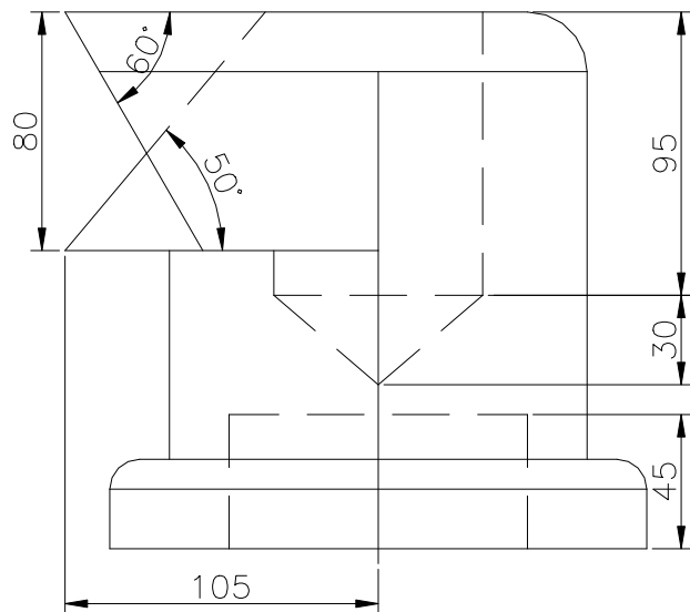
FRONT SCALE 1/3
