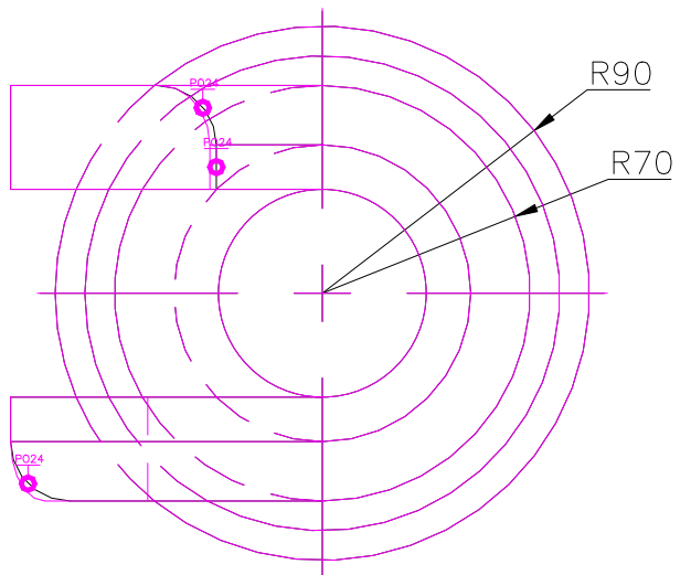
TOP SCALE 1/3
