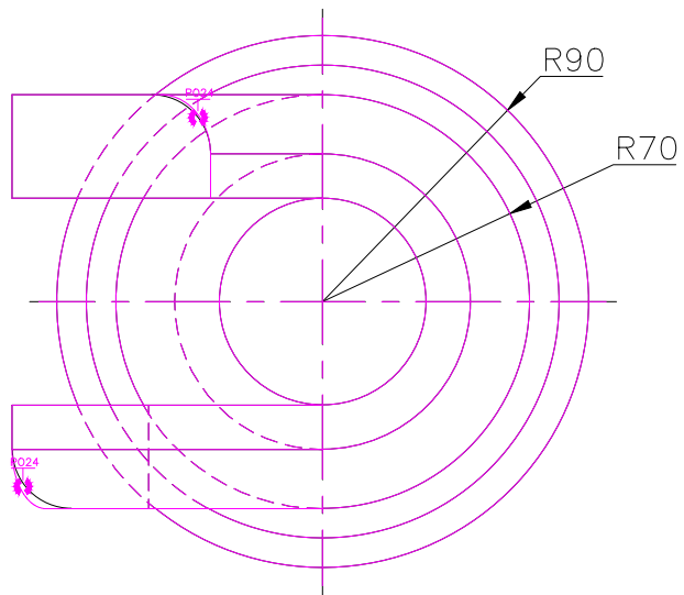
TOP SCALE 1/3
