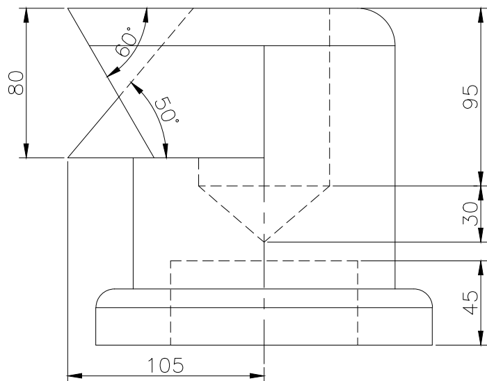
FRONT SCALE 1/3
