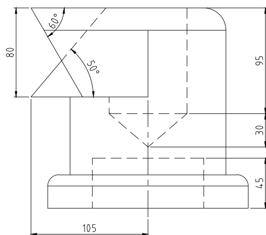
FRONT SCALE 1/3
