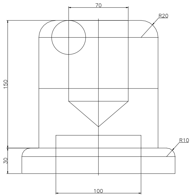
RIGHT SCALE 1/3
