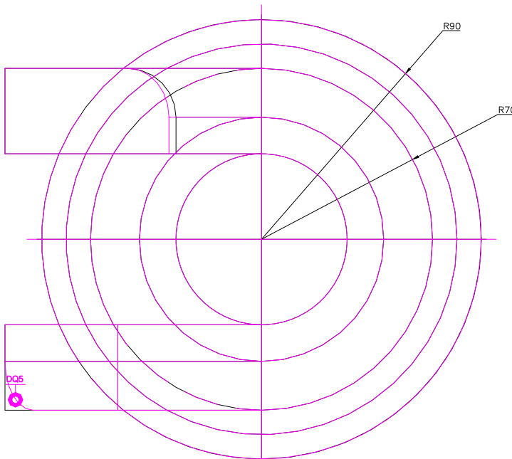
TOP SCALE 1/3
