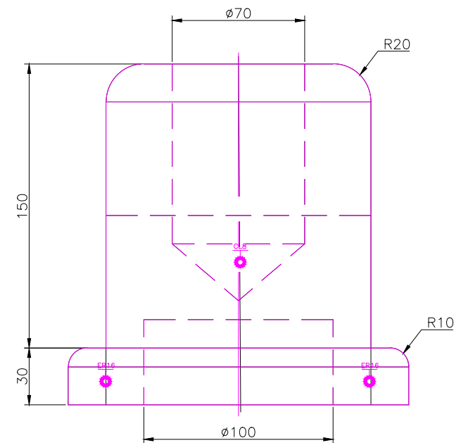
RIGHT SCALE 1/3
