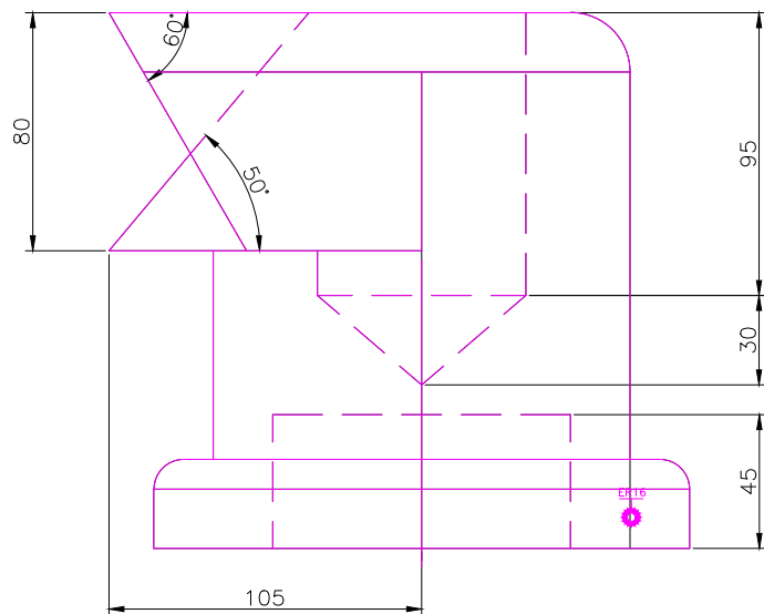
FRONT SCALE 1/3
