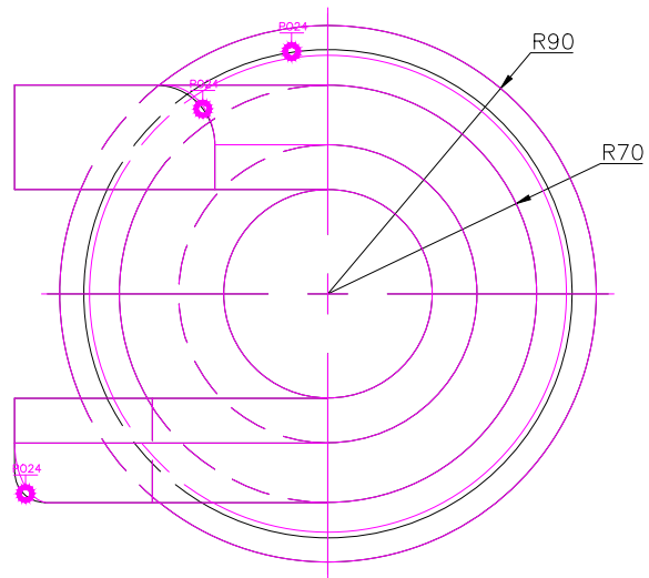
TOP SCALE 1/3
