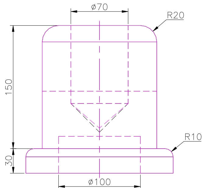
RIGHT SCALE 1/3
