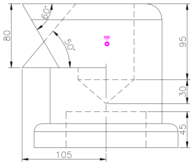
FRONT SCALE 1/3
