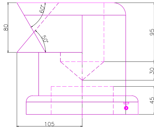
FRONT SCALE 1/3
