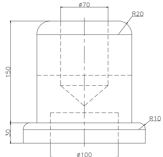
RIGHT SCALE 1/3
