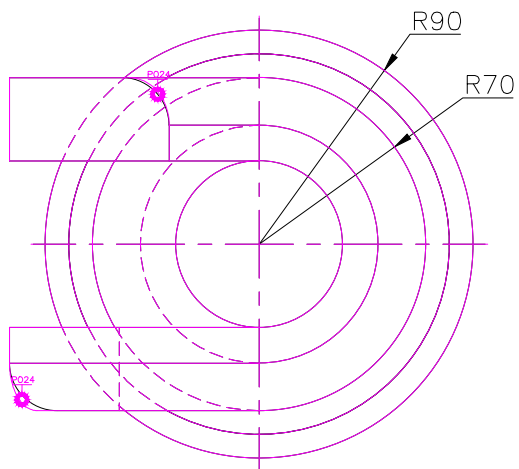
TOP SCALE 1/3
