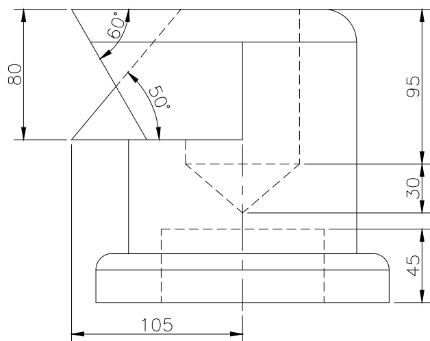
FRONT SCALE 1/3
