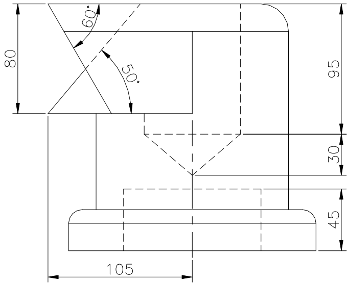
FRONT SCALE 1/3
