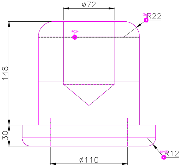
FRONT SCALE 1/3
