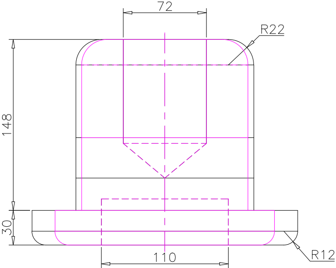
FRONT SCALE 1/3
