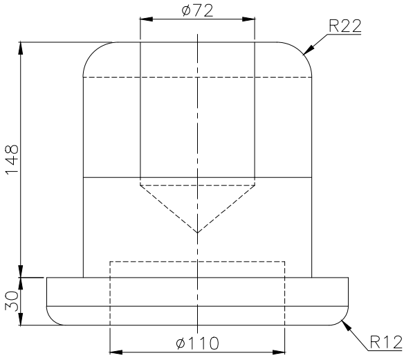
FRONT SCALE 1/3
