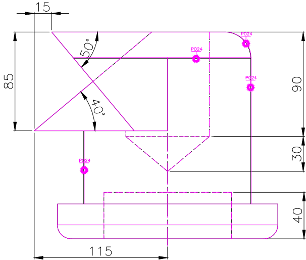
RIGHT SCALE 1/3
