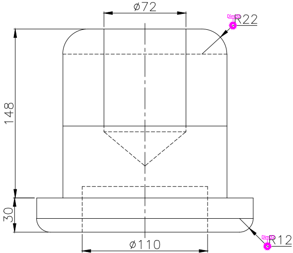
FRONT SCALE 1/3
