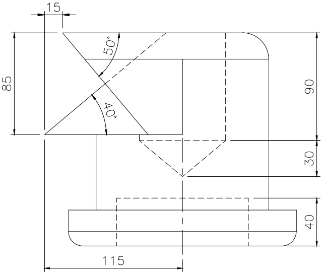
RIGHT SCALE 1/3
