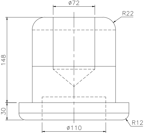
FRONT SCALE 1/3
